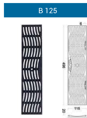
Ductile Iron Grating
