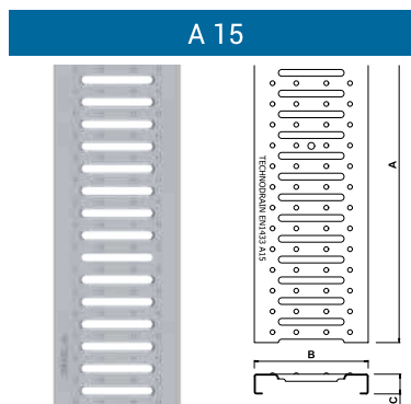
Galvanized Slotted Grating
