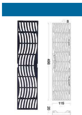
HDPE Black Grating
