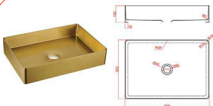
PWB 03 Bathroom Basin Rectangle
